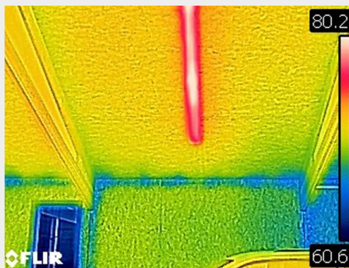
IMAGE 1.6: SIP GARAGE WITH LOW THERMAL BRIDGING IN WALL/ROOF
