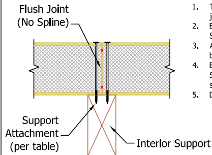
FIGURE A - INTERIOR SUPPORT
