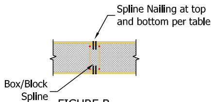
FIGURE B - BOX/BLOCK SPLINE
