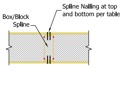
FIGURE B - BOX/BLOCK SPLINE
