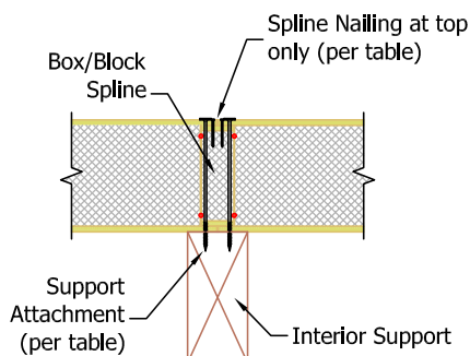
FIGURE A - INTERIOR SUPPORT
