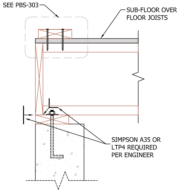
C: HANGING FLOOR SYSTEM
