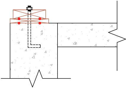
C: WALL AND SLAB ON GRADE
