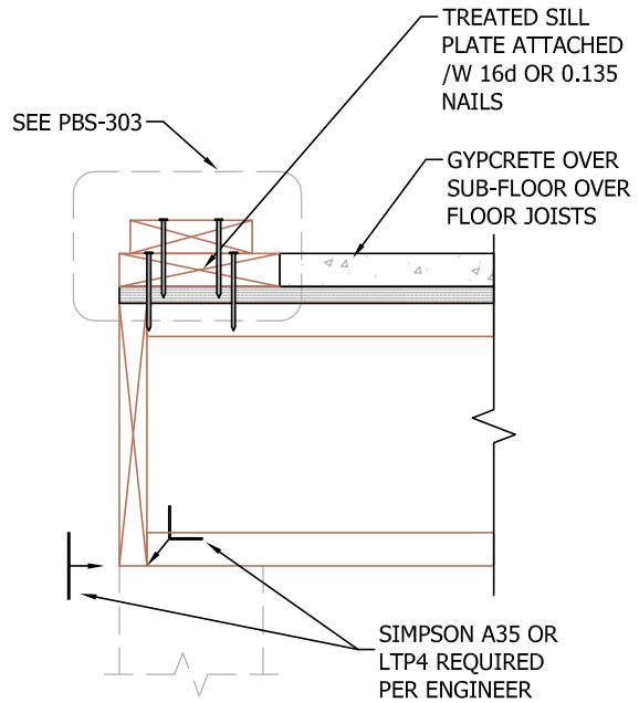
H: HANGING FLOOR SYSTEM
